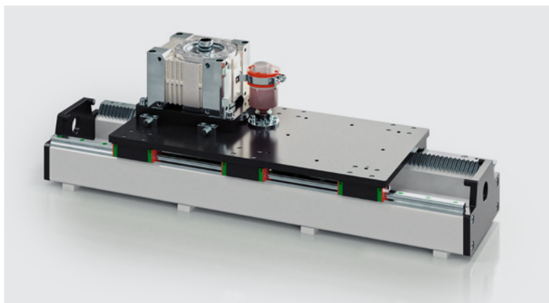
KK-RP - Rack and pinion
