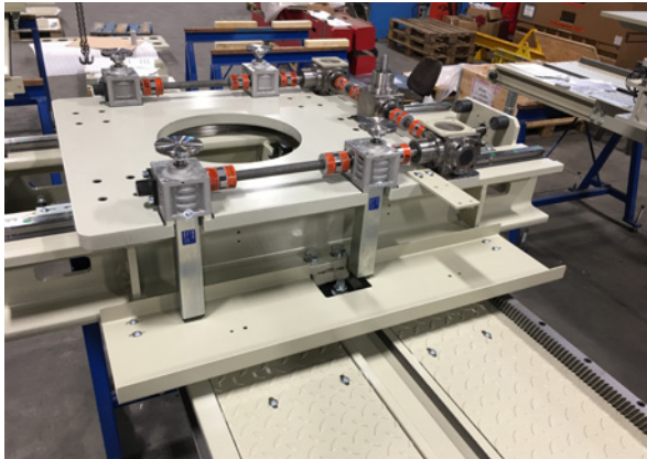
X-Y-Z - Positioning system for an extruder
